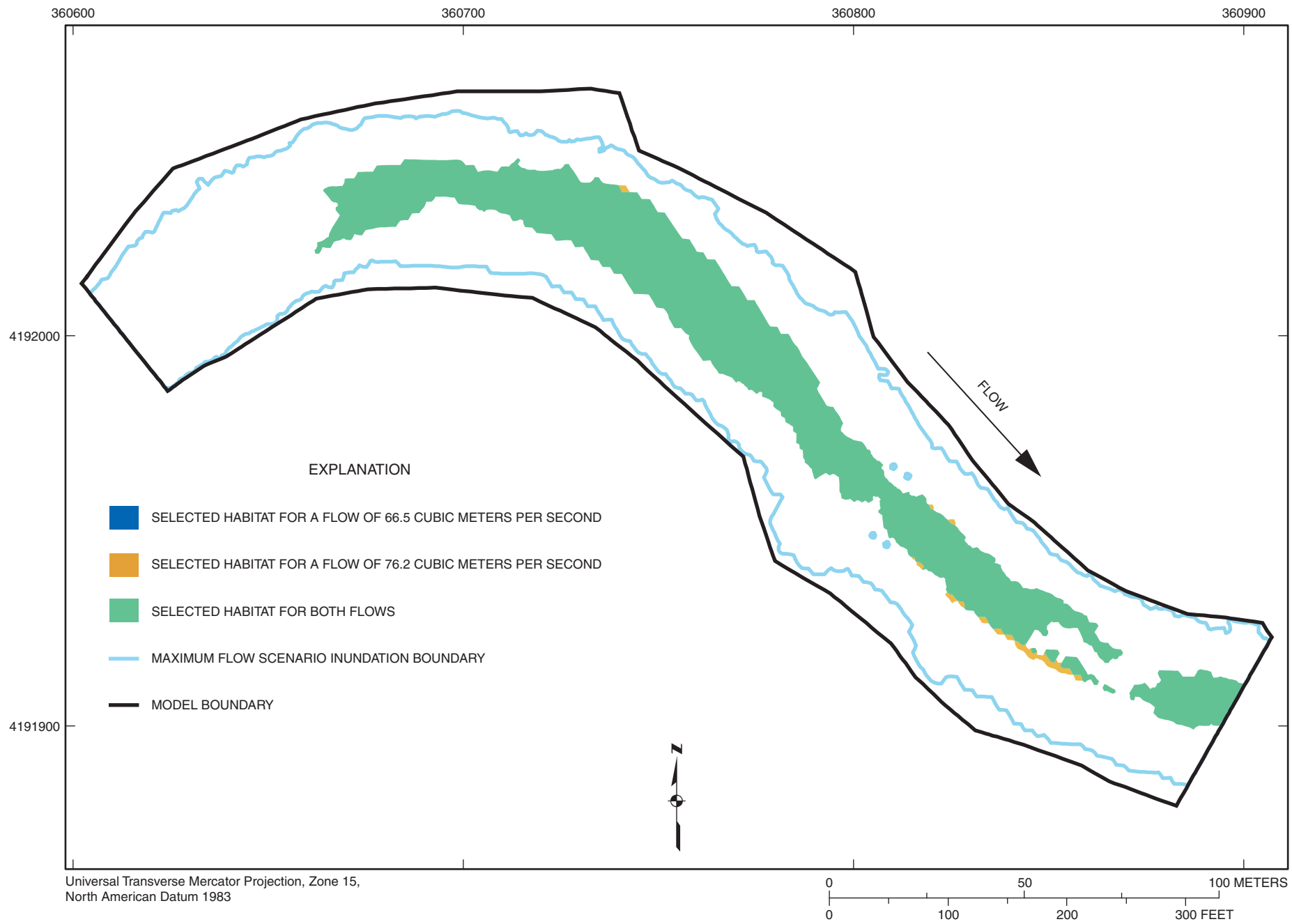
Figure 1-23. Selected habitat area distribution for habitat category 7 (paddlefish) at flows of 66.5 and 76.2 cubic meters per second at Marmaton River site M1.
